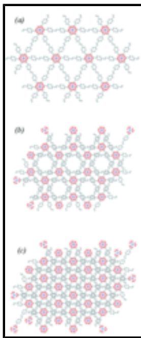
Fig. 2. [001] view of the structure showing the 3^6 topology. (a) A single 2D layer. (b) Two overlapped close-packed layers, A and B. (c) Cubic close-packed layers, in ABC pattern.
